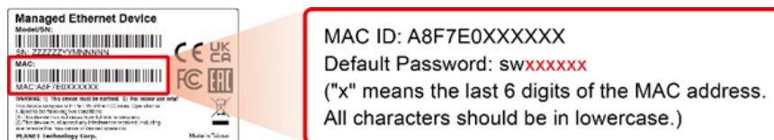
Figure 7-3: MAC ID Label
