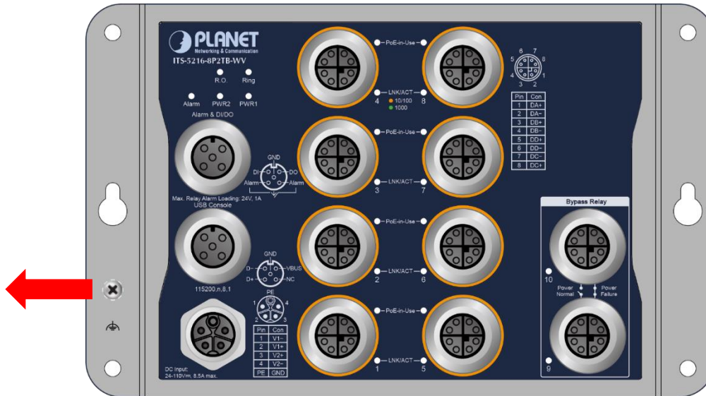
Figure 5-1: ITS-5216 Series Earth Grounding
