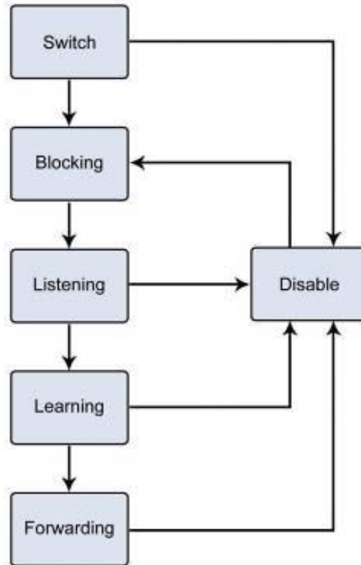
Figure 4-6-1: STP Port State Transitions
