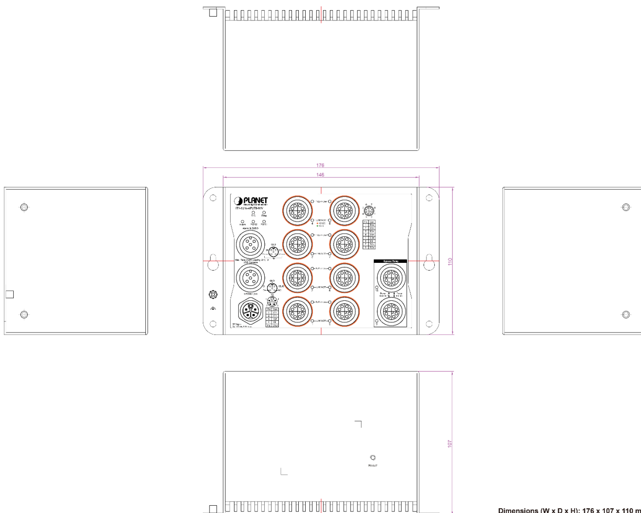
Dimensions (W x D x H): 176 x 107 x 110 mm
