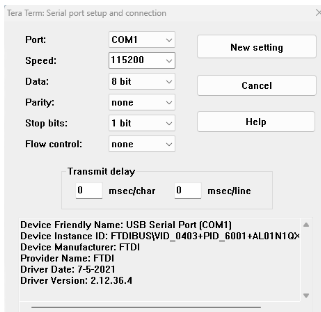
Figure 7-2: COM Port Configuration
