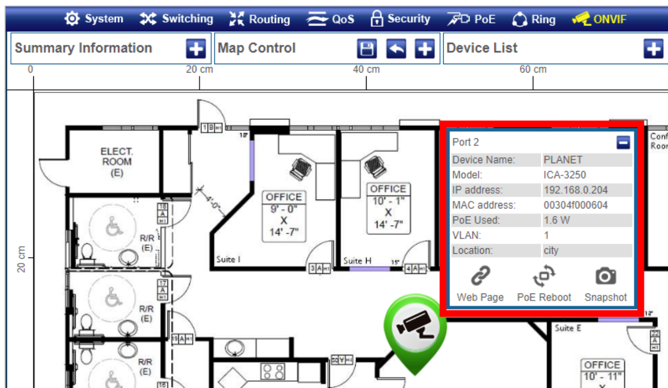
Figure 4-16-7: Floor Map Page Screenshot – Display device information of selected ONVIF IP camera
