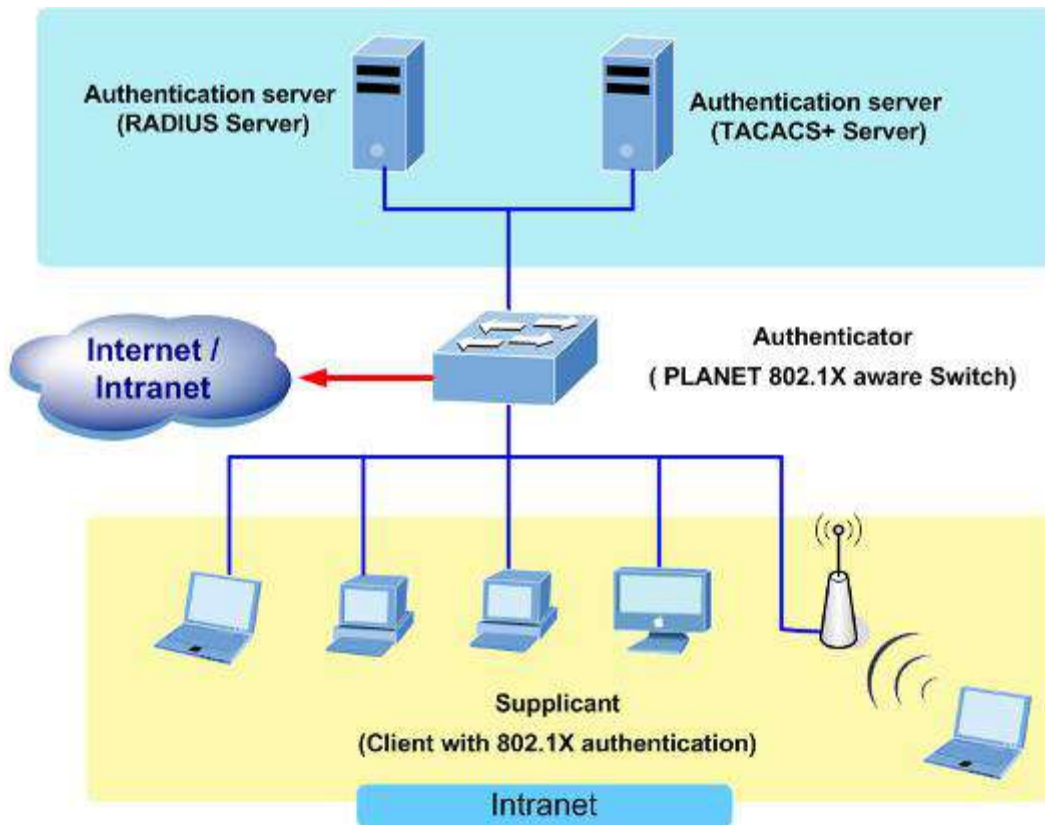
Figure 4-13-4-1
