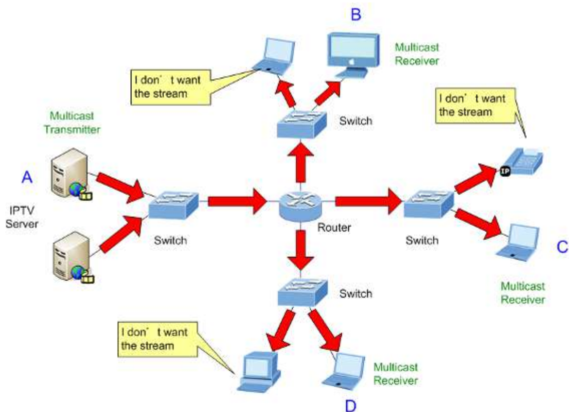
Figure 4-8-2: Multicast Flooding
