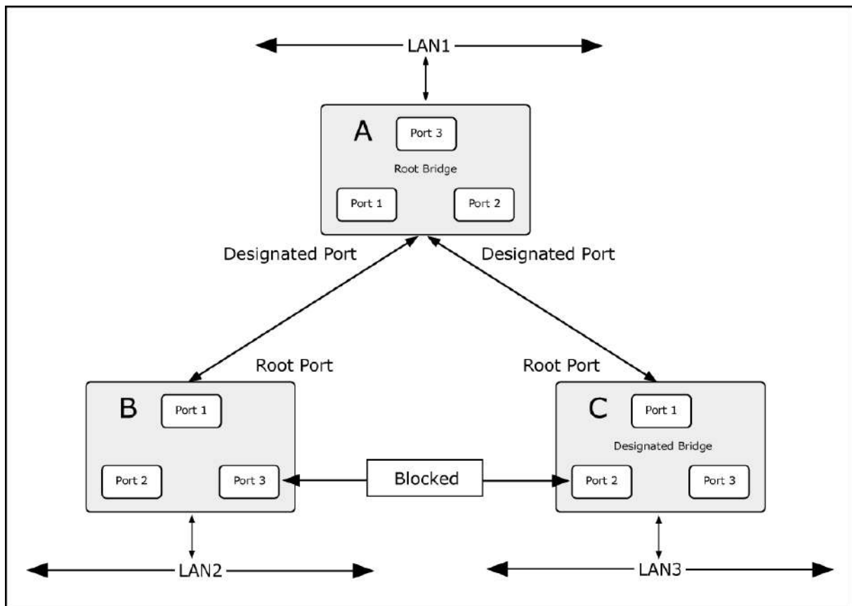
Figure 4-6-1-2: After Applying the STA Rules
