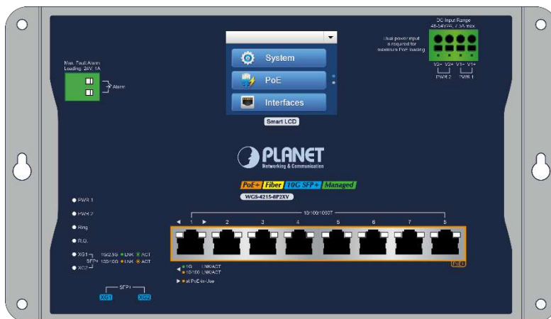
Figure 2-1-1: Front Panel of WGS-4215-8P2XV
