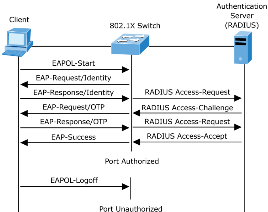
Figure 4-13-4-2: EAP Message Exchange
