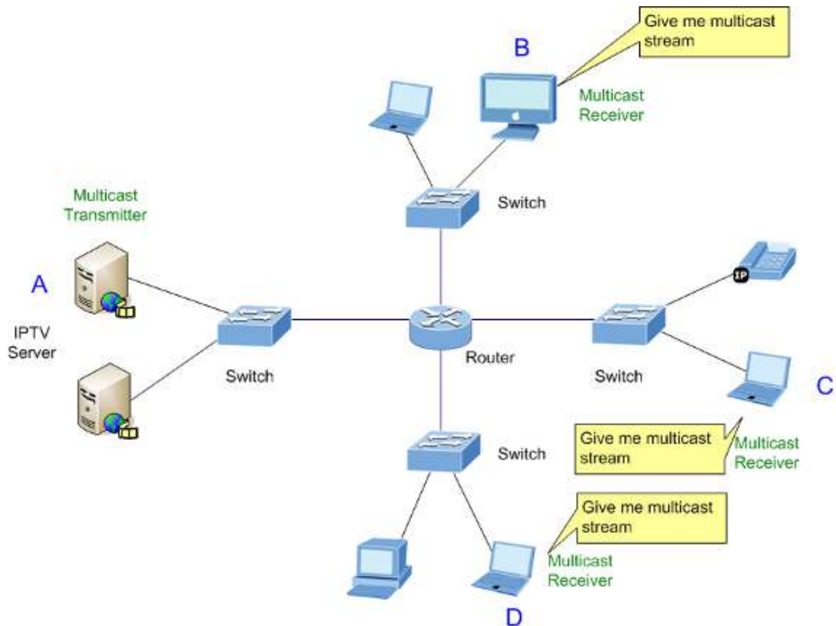
Figure 4-8-1: Multicast Service
