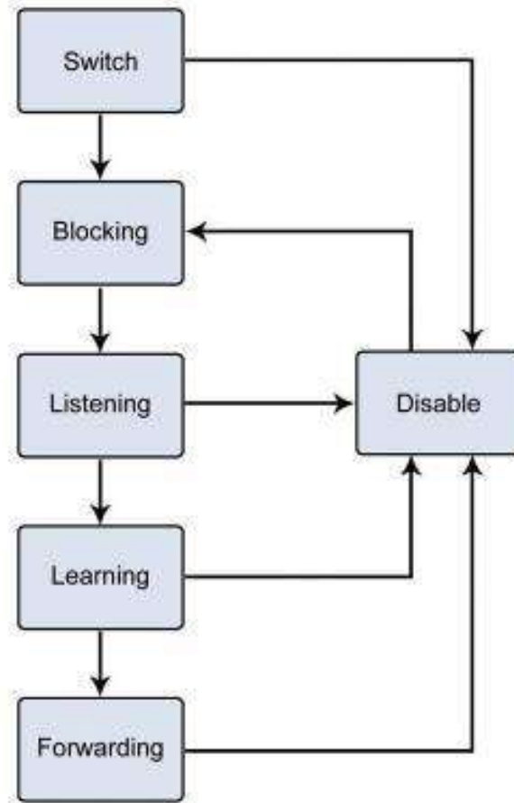
Figure 4-6-1-1: STP Port State Transitions
