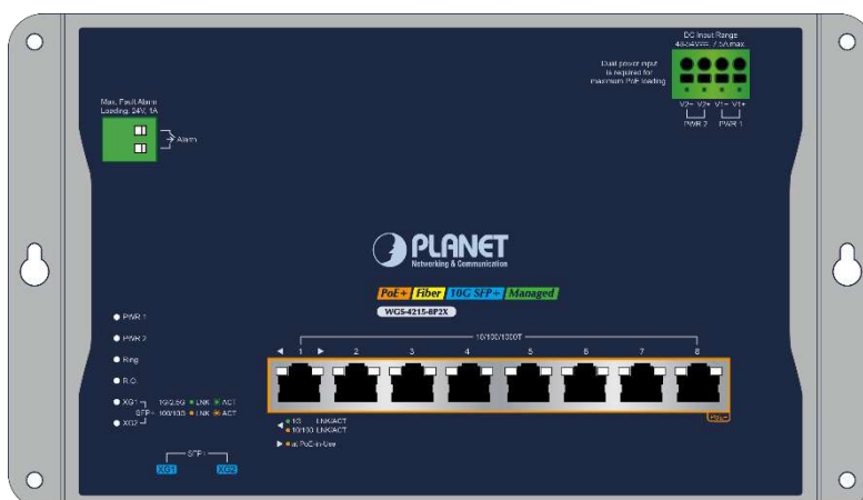
Figure 2-1-2: Front Panel of WGS-4215-8P2X
