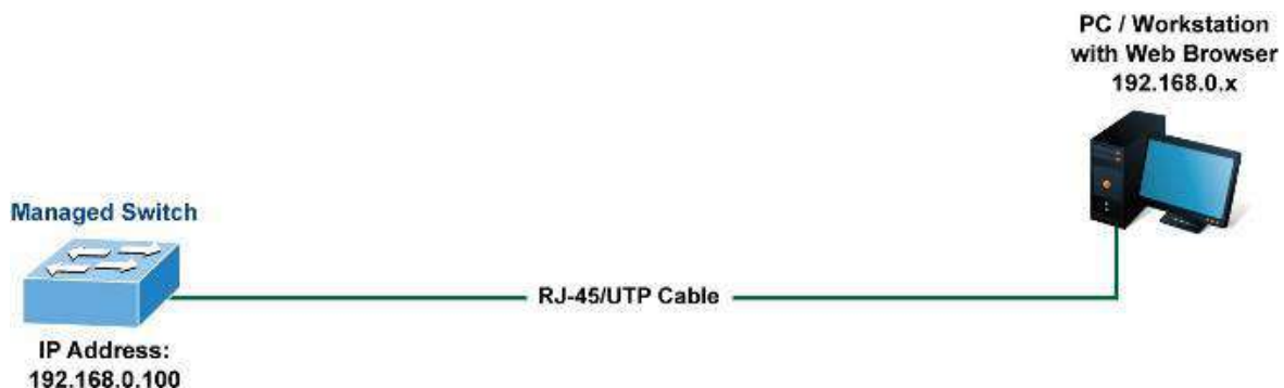
Figure 4-1: Web Management
