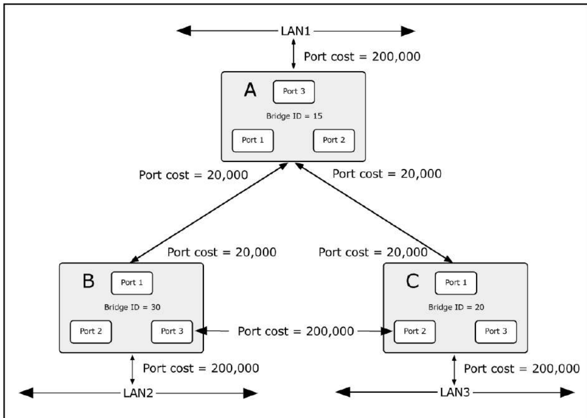
Figure 4-6-1-2: Before Applying the STA Rules
