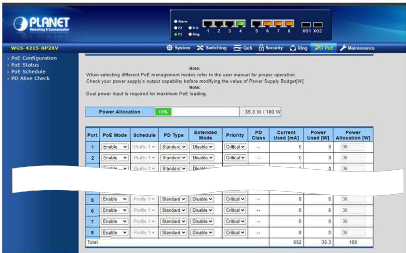
Figure 4-15-1-1: Power over Ethernet Status
