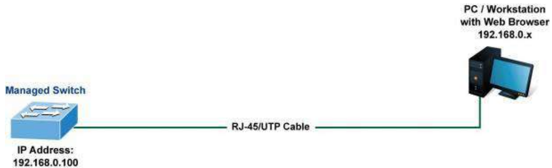
Figure 3-3-1: Web Management
