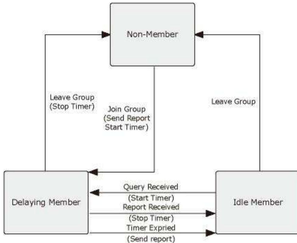
Figure 4-8-4: IGMP State Transitions
