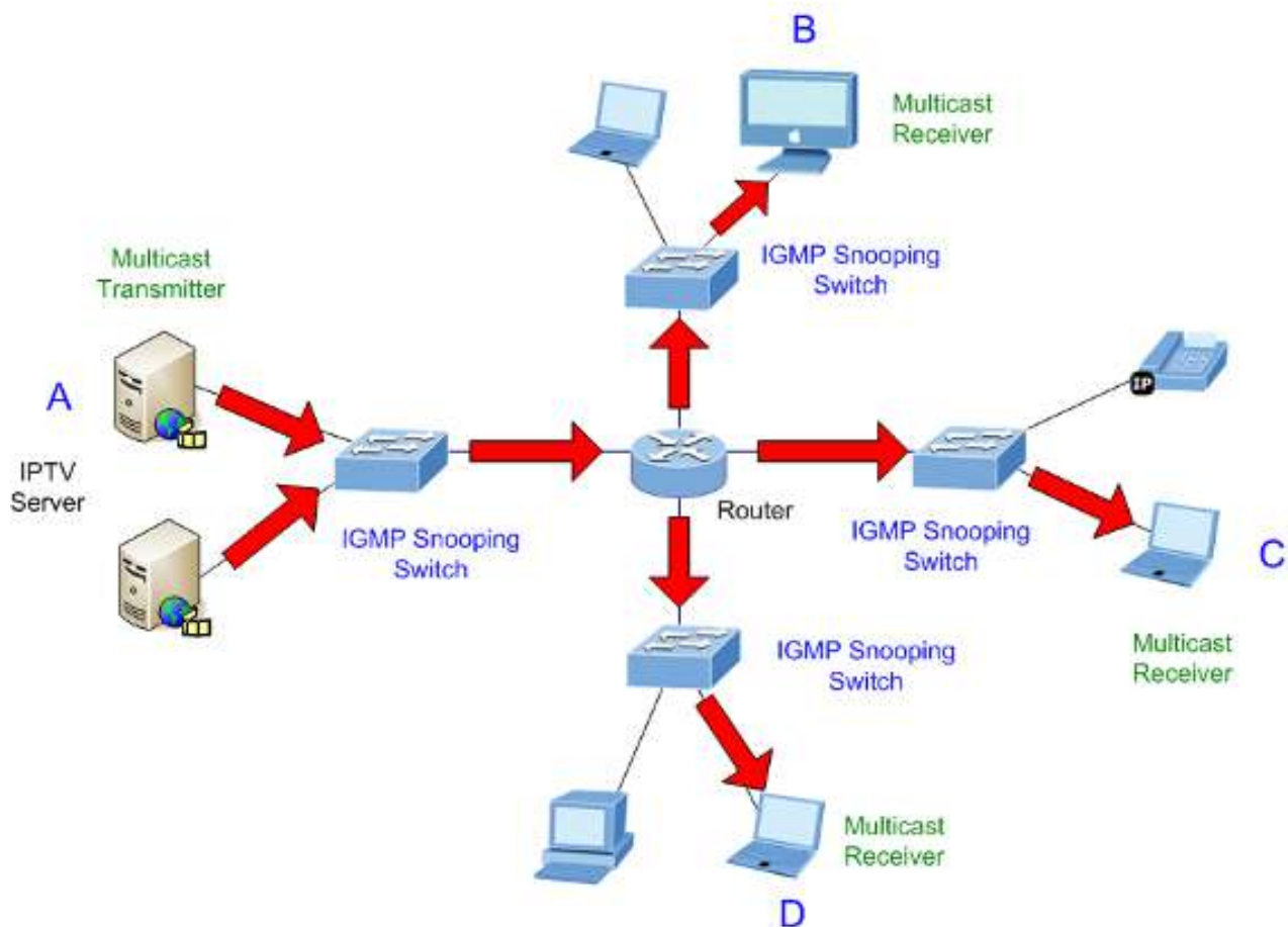
Figure 4-8-3: IGMP Snooping Multicast Stream Control
